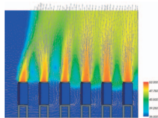
CFD Simulation
